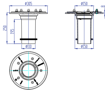
Art. no. 7040.12.02 Corp izolator extensie
