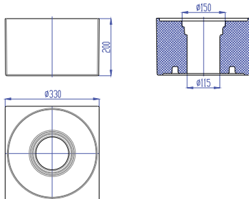
Art. no. 7040.12.02 Corp izolator extensie
