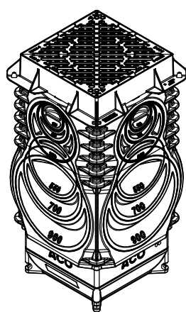
ISOMETRIC VIEW SCALE 1:20
