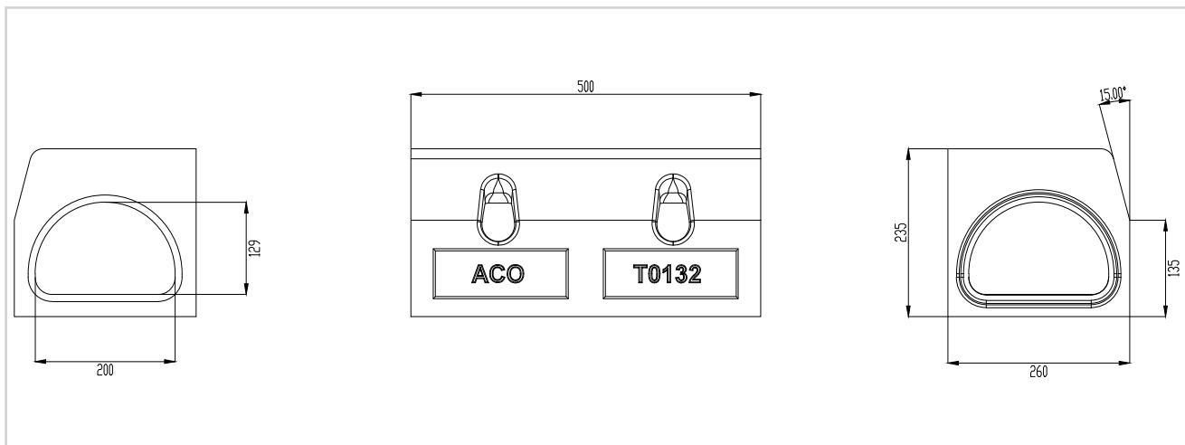
Kerb Drain® Bridge Drain 235 mm
