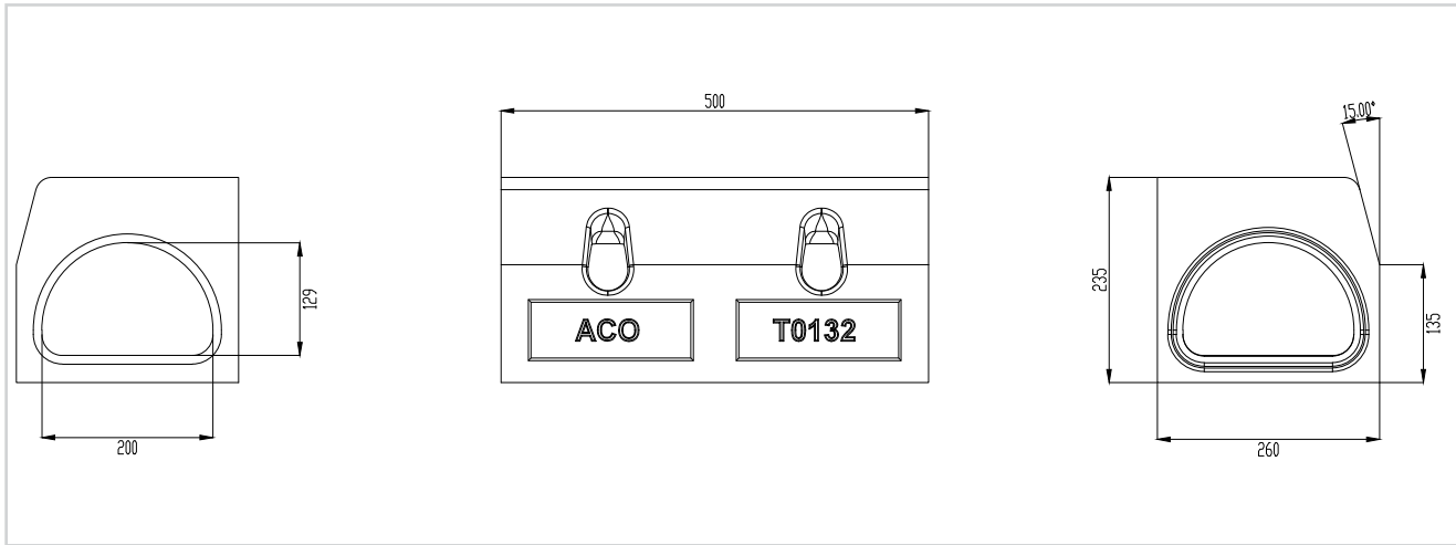
Kerb Drain® Bridge Drain 235 mm
